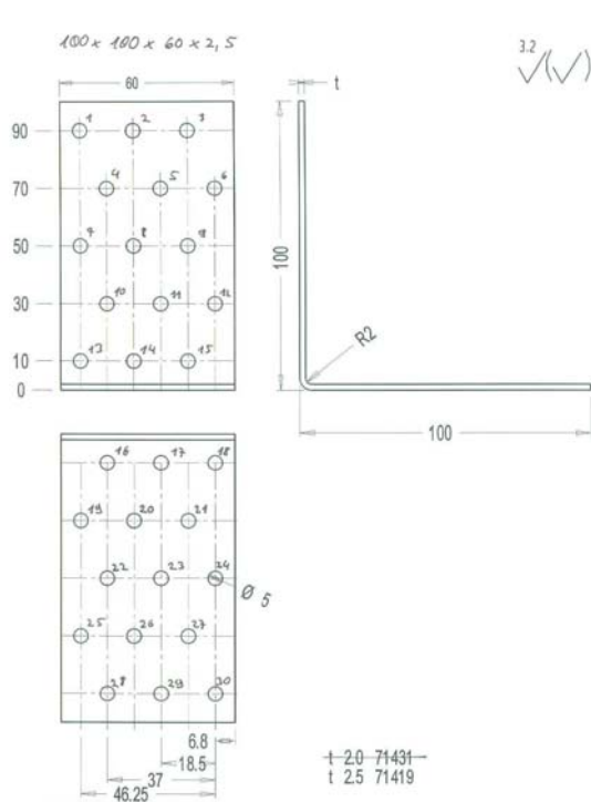
Figure B. 68 Dimensions of angle bracket
