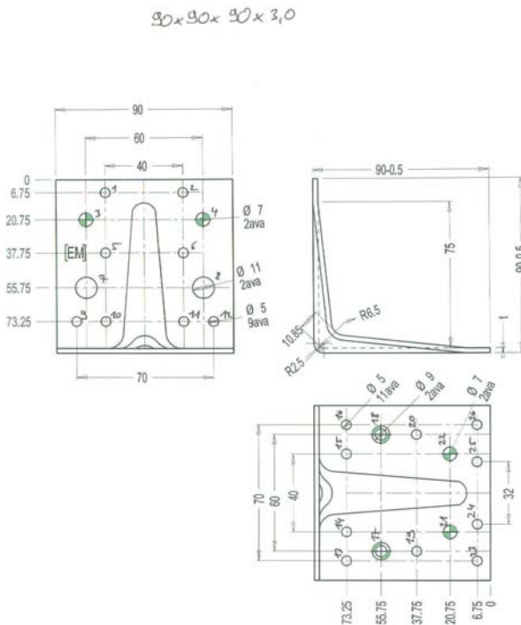
Figure B. 60 Dimensions of angle bracket
