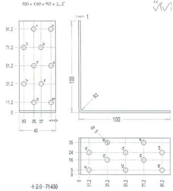
Figure B. 63 Dimensions of angle bracket
