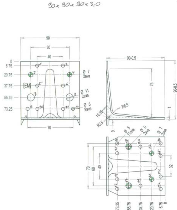
Figure B. 61 Dimensions of angle bracket
