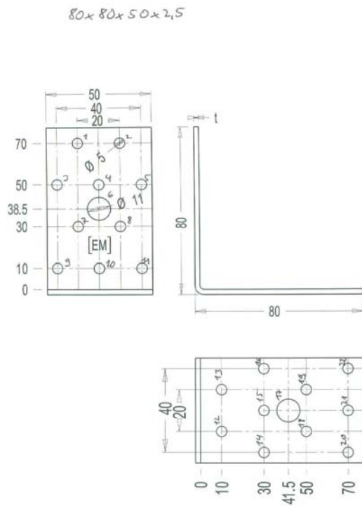
Figure B. 42 Dimensions of angle bracket
