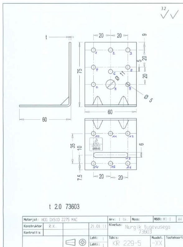
Figure B.34 Dimensions of angle bracket
