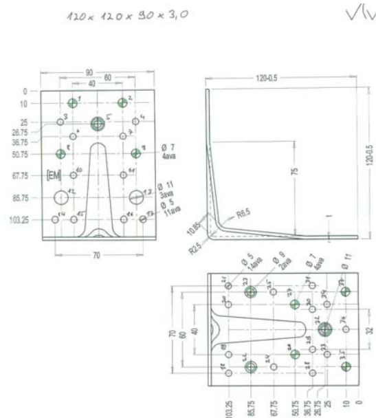
Figure B. 81 Dimensions of angle bracket
