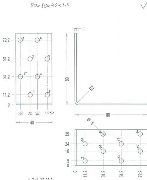
Figure B. 40 Dimensions of angle bracket
