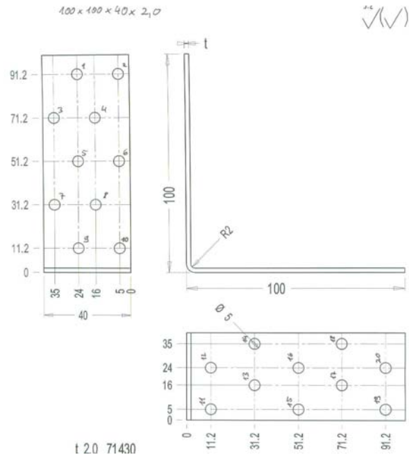
Figure B. 62 Dimensions of angle bracket
