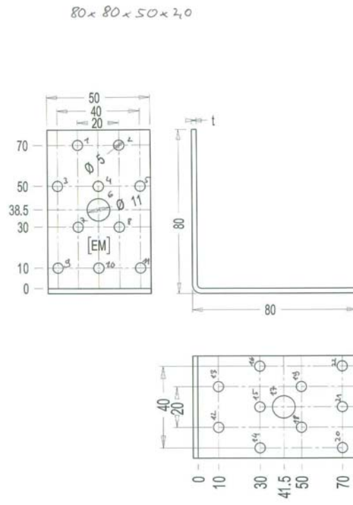
Figure B. 41 Dimensions of angle bracket
