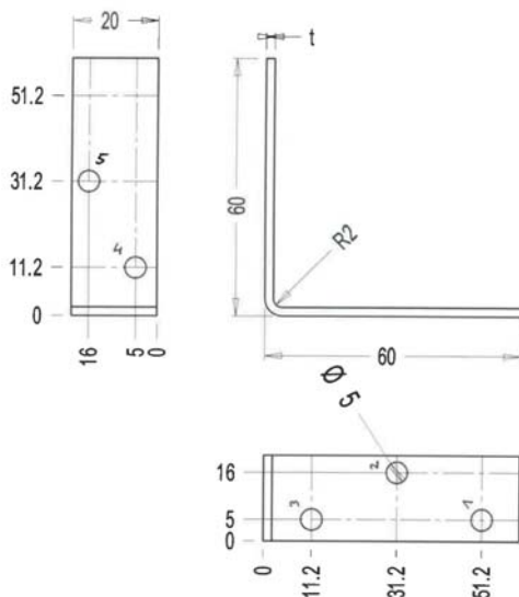
Figure B. 15 Dimensions of angle bracket
