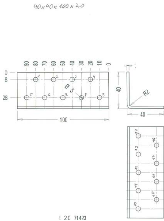
Figure B. 9 Dimensions of angle bracket
